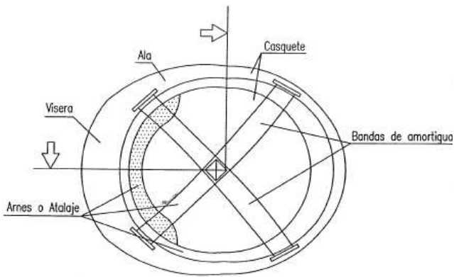
CASCO - PROTECTOR AURICULAR
