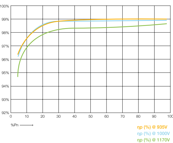
Efficiency PV 2250
