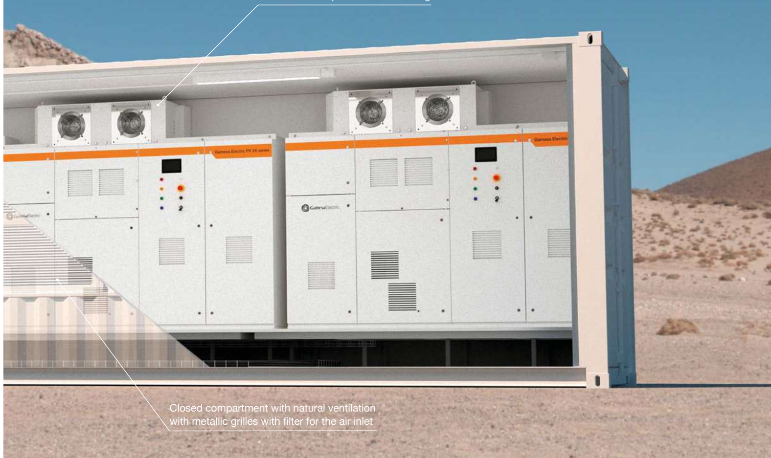
Gamesa Electric PV 2X series inverters with liquid/air active cooling
