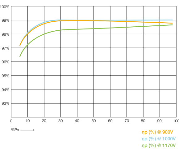
Efficiency PV 2500
